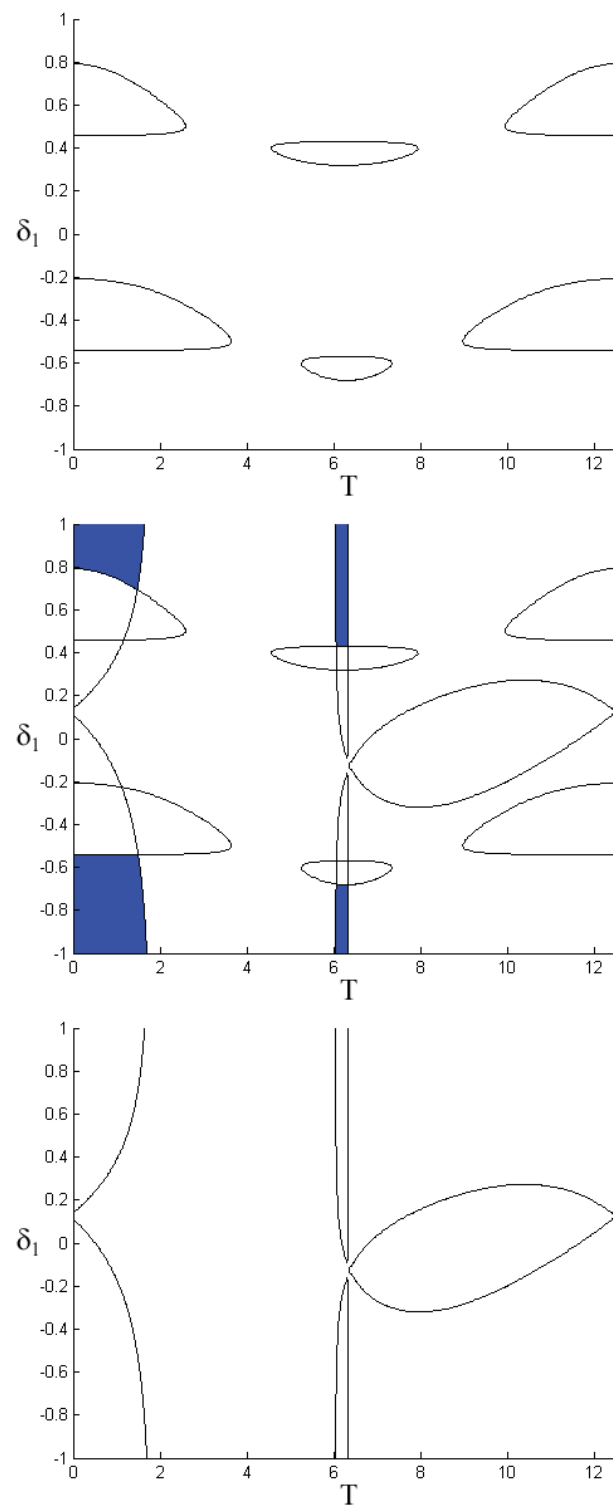
Fig. 1 The top graph shows the transition curves for the saddle node bifurcations of the non-delayed system ( \varepsilon = 0 ). The bottom graph shows the transition curves for the Hopf bifurcations of the non-delayed system ( \varepsilon = 0 ). The middle graph shows both sets of transition curves and has the stable regions shaded in. Parameter values are: \alpha = 0.1 ; \beta = 0.125 ; \mu = 0.01 .
