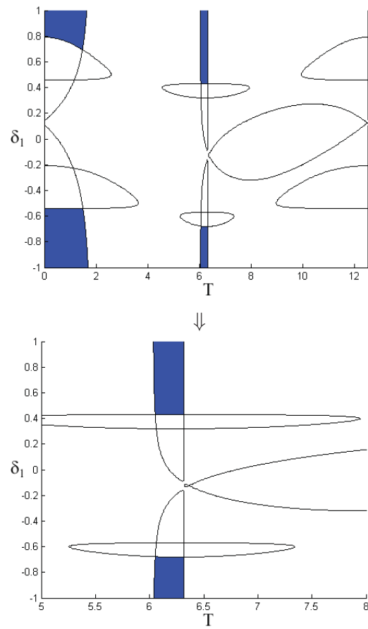
Fig. 2 The top graph is Figure 1. The bottom graph zooms in on the region for T between 5 and 8, while keeping the range of \delta_1 values the same.
