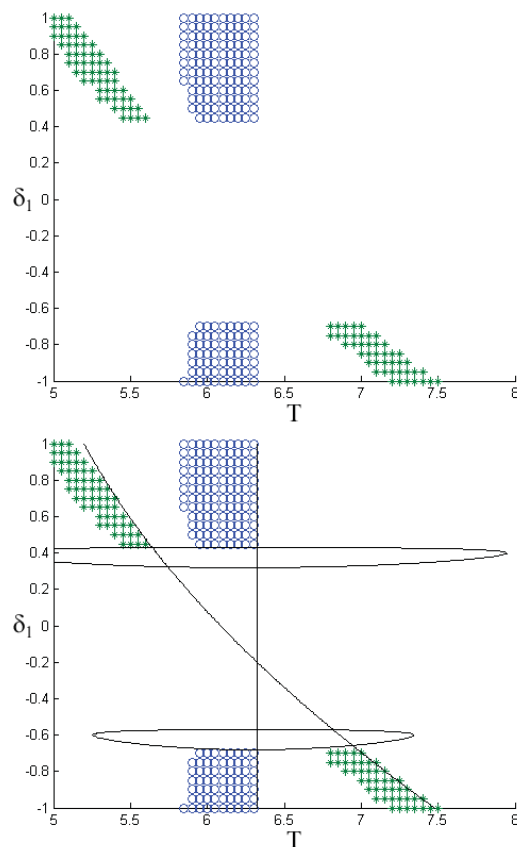
Fig. 4 The top graph shows the stable points near the Hopf curve as computed through numerical integration of the slow flow, with the circles representing the non-delayed system and the asterisks representing the delayed system. The bottom graph shows the Hopf and saddle node transition curves on top of these stable regions.
