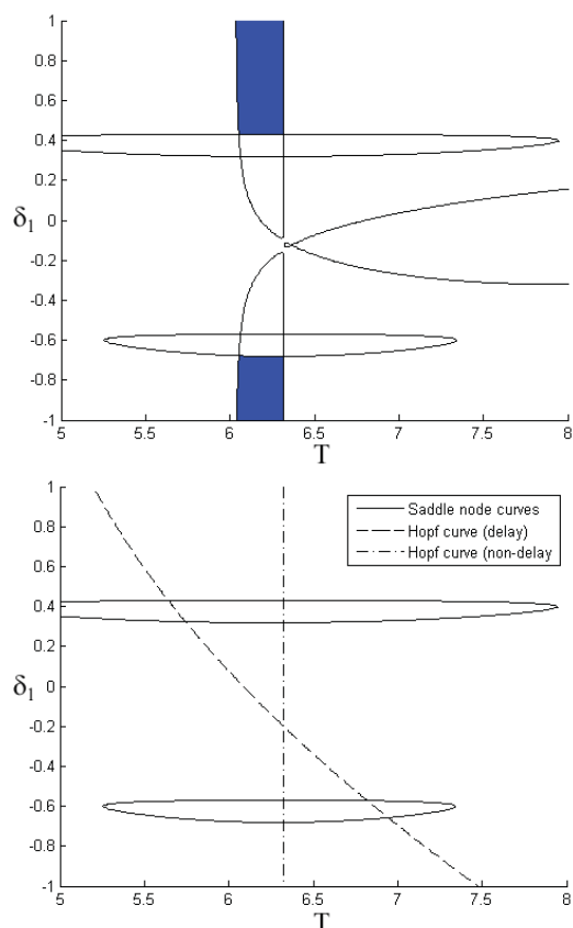
Fig. 3 The top graph is the blowup of Figure 1. The bottom graph shows the series solutions for the Hopf curves for both the delayed and non-delayed systems, as well as the saddle node bifurcation curves.
