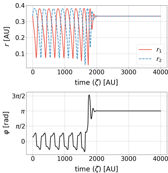
Fig. 12 Slow flow system starting on the separatrix at \alpha = 0.042 and going over to the OP mode
