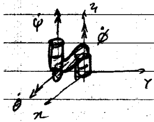
Figure 9.9: Singular x-z-x Euler angle configuration, also known as Gimbal lock.
