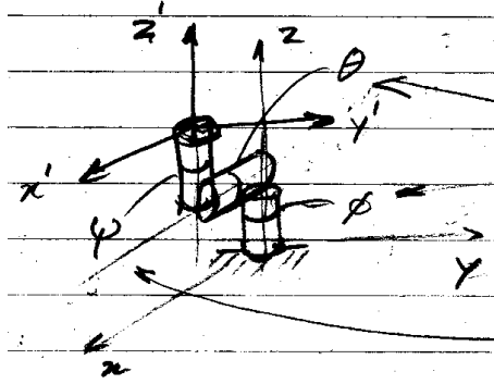
Figure 9.3: Euler angles x - z - x denoted by \phi, \theta, \psi depicted by the so-called "cans in series" to show the order of rotation.
