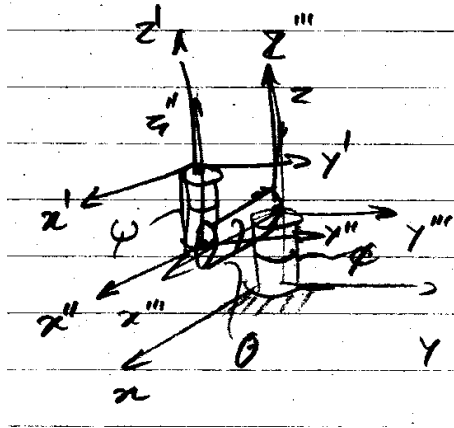
Figure 9.4: Euler angles x - z - x depicted by cans in series, together with the three individual rotations \phi, \theta, \psi and corresponding ''', '' and ' coordinate systems.
