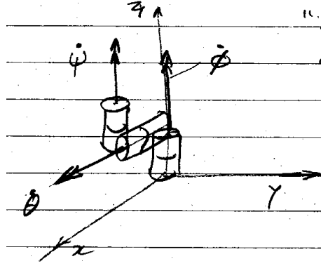
Figure 9.7: Sketch of the three velocity vectors for the three x - z - x Euler angles \phi, \theta, \psi .
