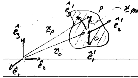
Figure 9.6: Sketch fixed and body fixed coordinate system
